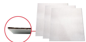
Cushion: CU-003 (size: 360x360x1mm)
